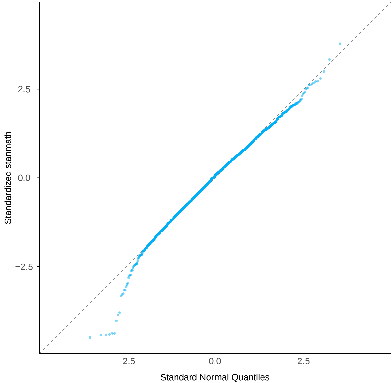
Normal Q-Q: stanmath
