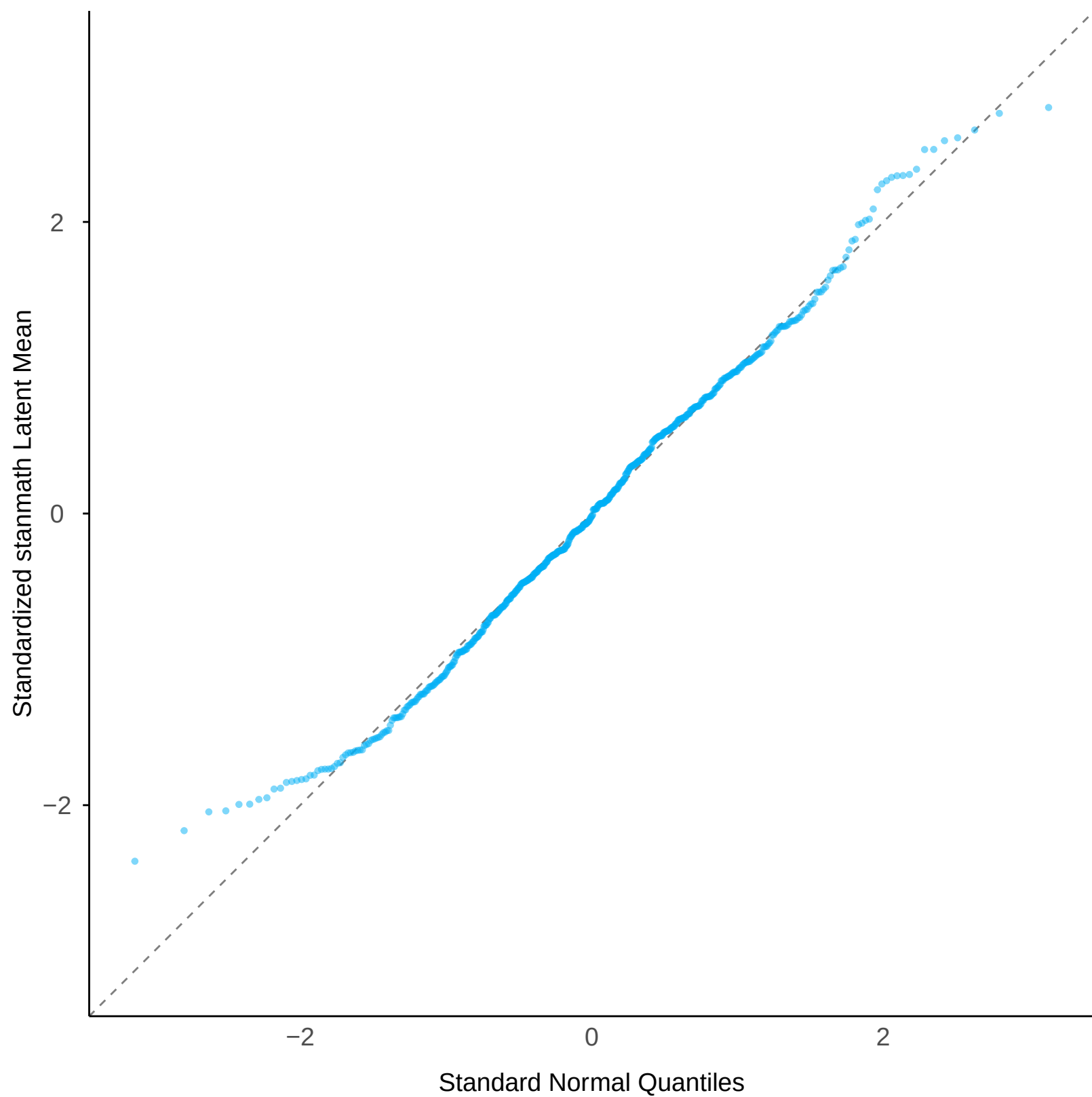
Normal Q-Q: stanmath Latent Mean
