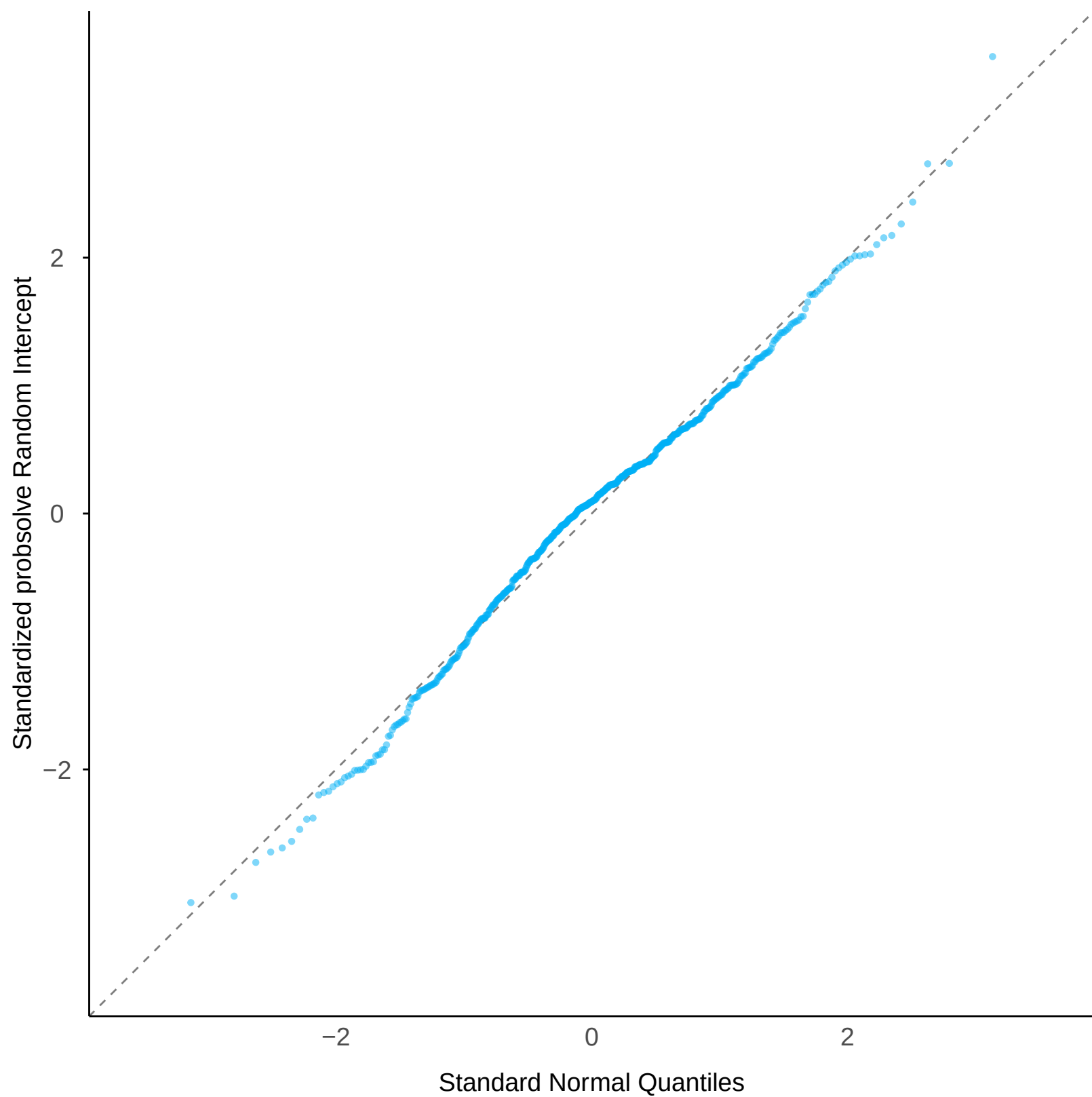
Normal Q-Q: probsolve Random Intercept
