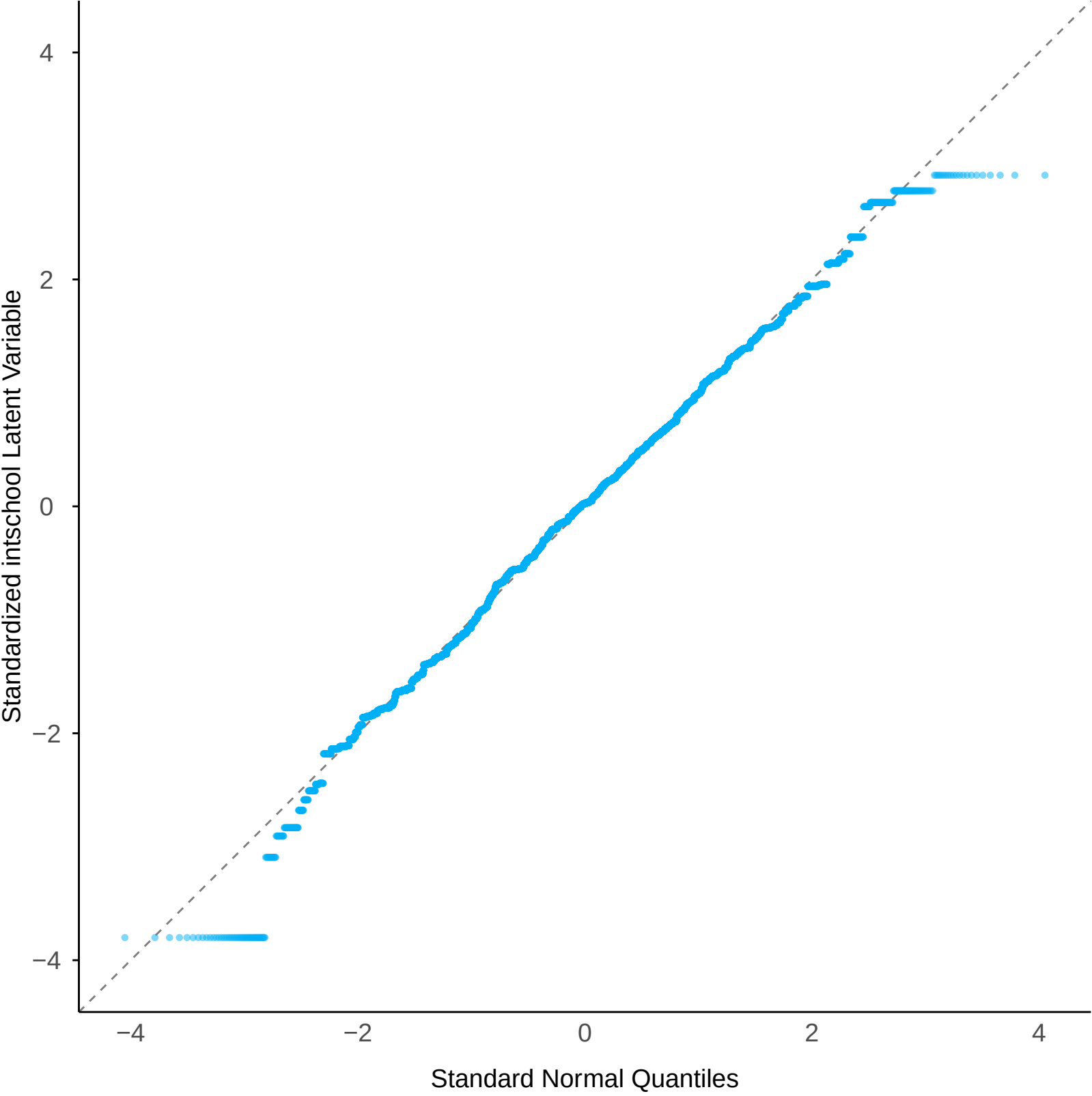
Normal Q-Q: intschool Latent Variable
