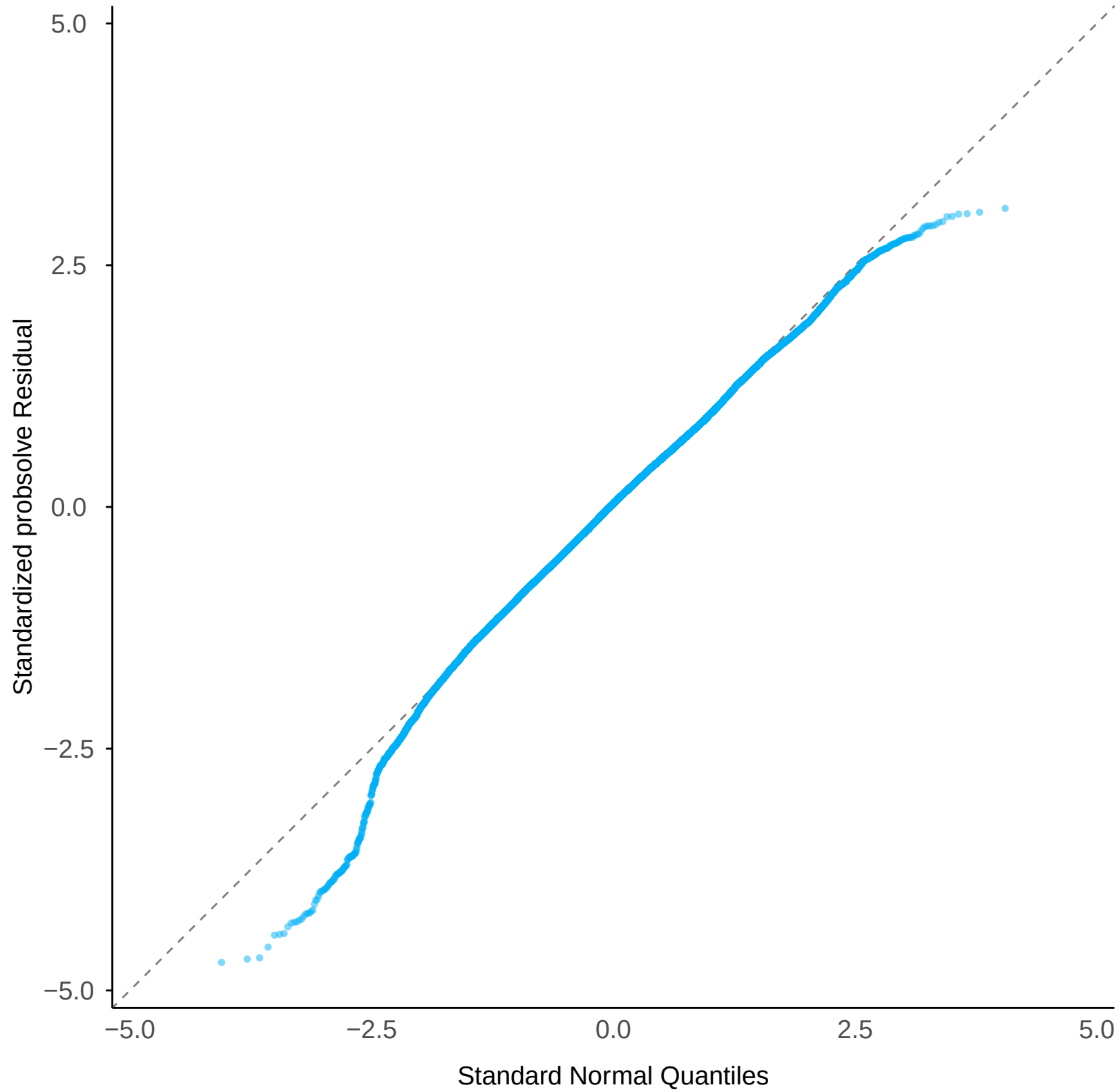
Normal Q-Q: probsolve Residual
