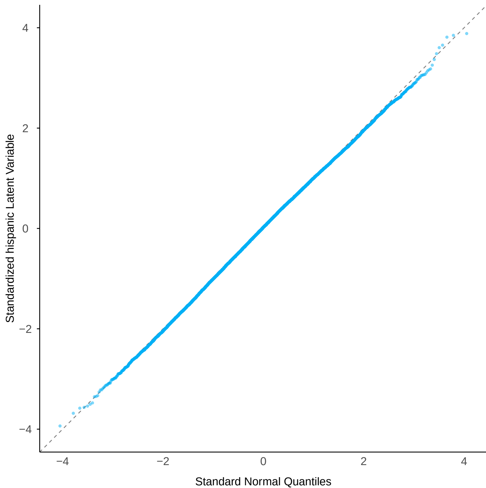
Normal Q-Q: hispanic Latent Variable
