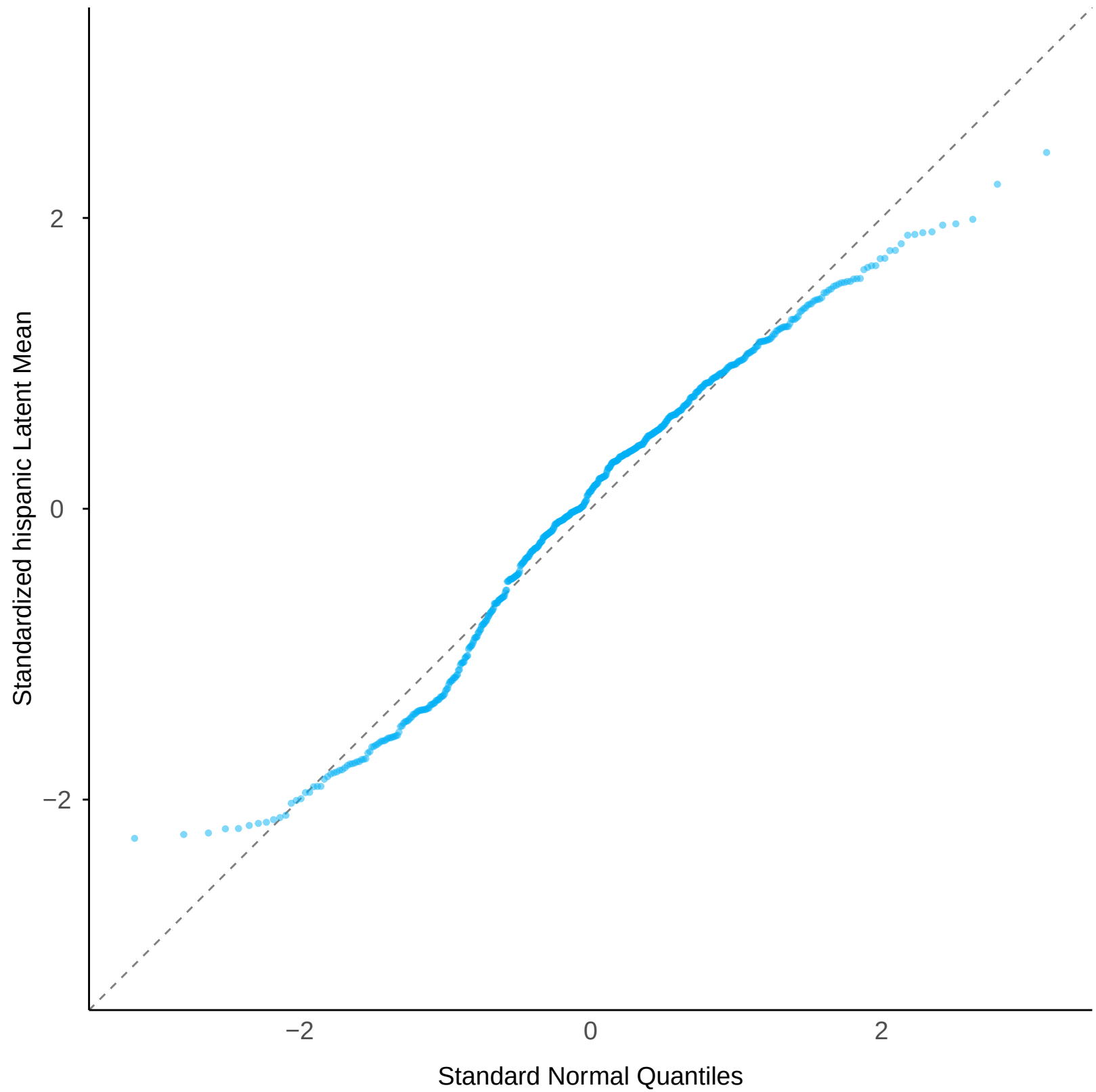
Normal Q-Q: hispanic Latent Mean
