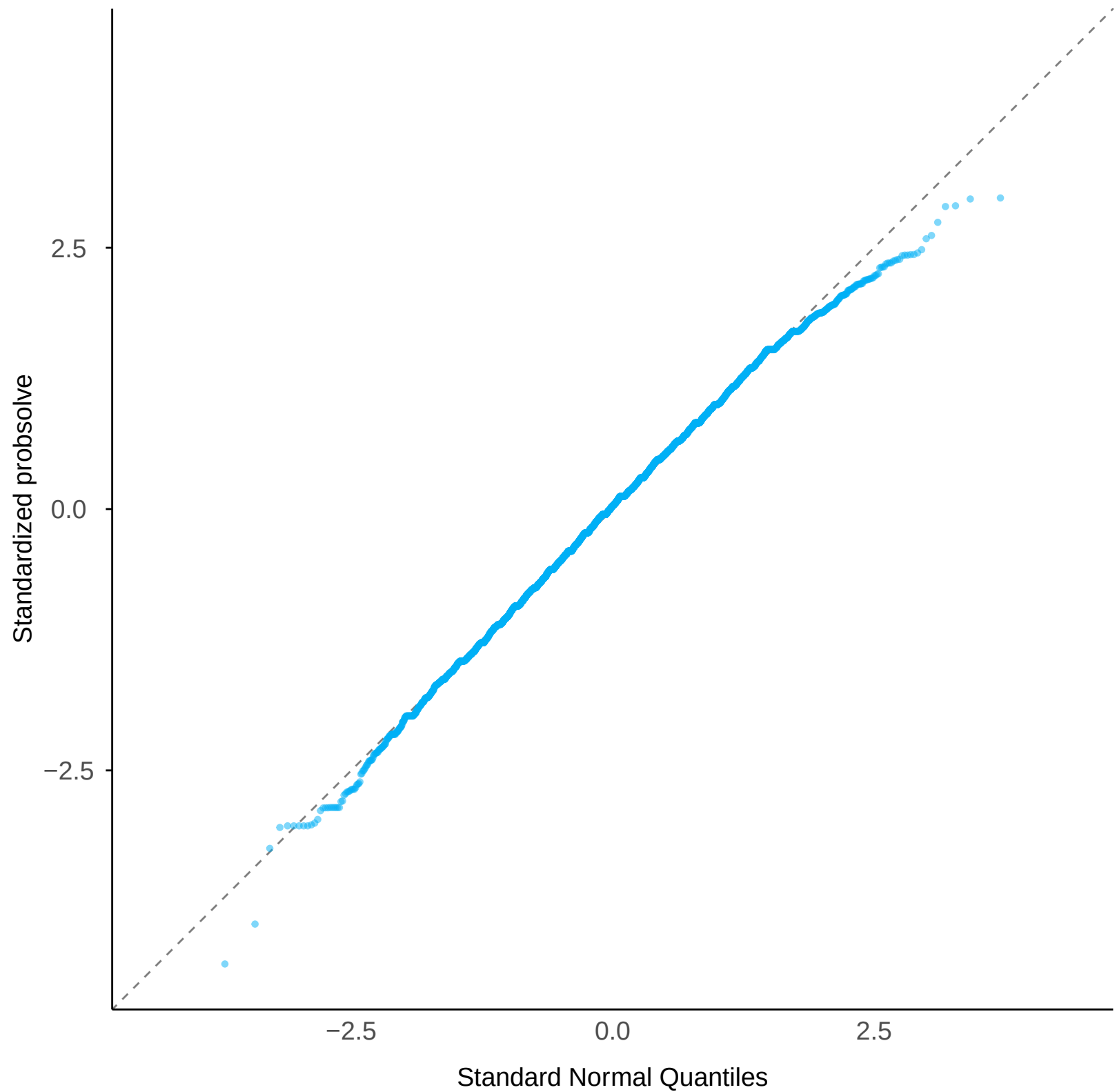
Normal Q-Q: probsolve
